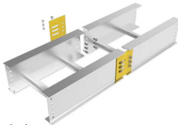
Expansion Coupler
