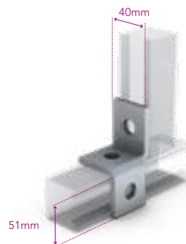
Right Hand Two Bend L Support
