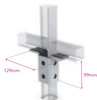
Two Leg Support
