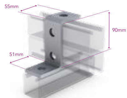
Deep Back to Back 'Z' Shaped Bar
