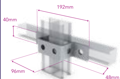
Back to Back Flat Top Hat Bracket
