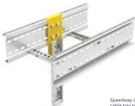
Speedway drop out bracket securing a vertical cable ladder to a horizontal cable ladder run
