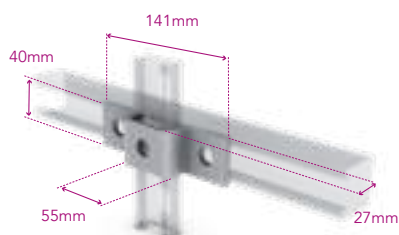
Shallow Normal Top Hat Bracket
