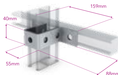
Back to Back Normal Top Hat Bracket
