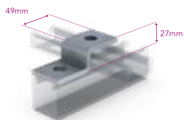
Shallow 'Z' Shaped Bracket
