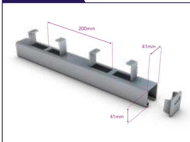
Ref. IC-CON-D
